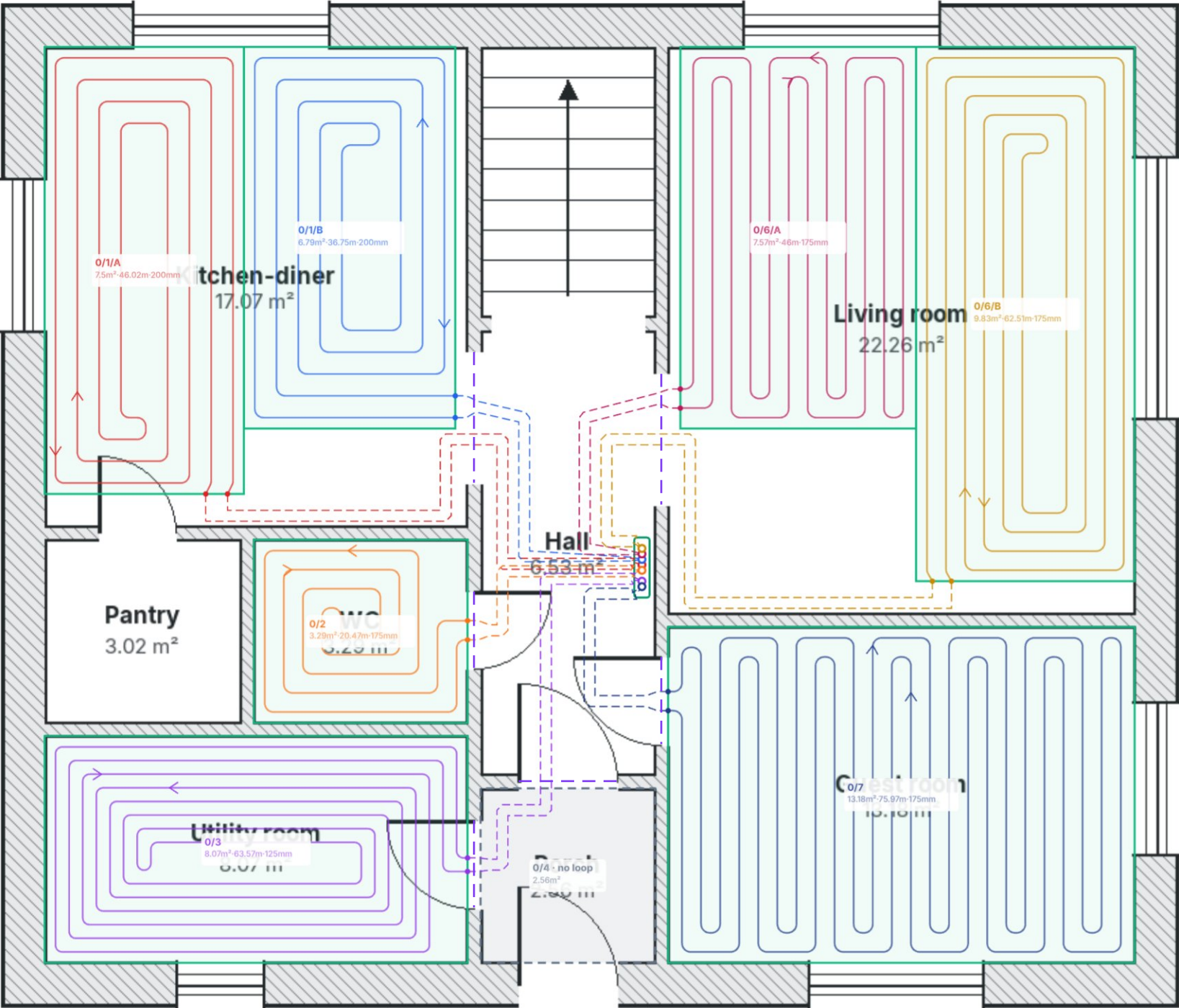
GROUND FLOOR
